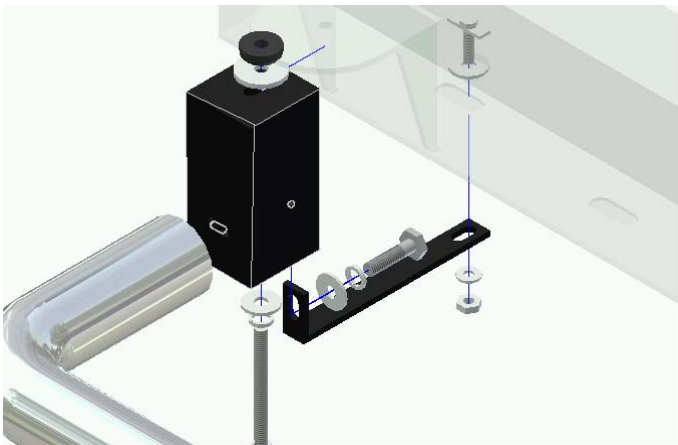
Figure 1.4 – 1500 Front Mount Assembly
